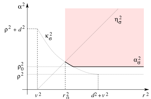
Figure 12: The simplex \sigma belongs to K(\alpha, r) iff the point (\alpha^2, r^2) lies in the shaded region above the function that discriminates between membership and non-membership.
