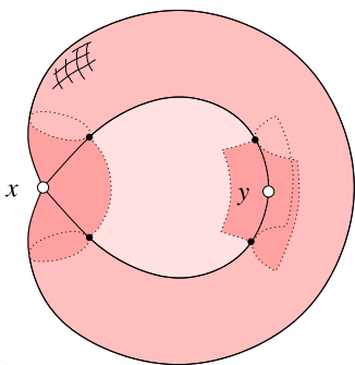
Figure 4: A 2-dimensional cs-space. The neighborhood of the pinch point x and of another point y along the boundary circle of the disk are highlighted. The two neighborhoods are not homeomorphic but they have the same homotopy type and therefore isomorphic homology groups.
